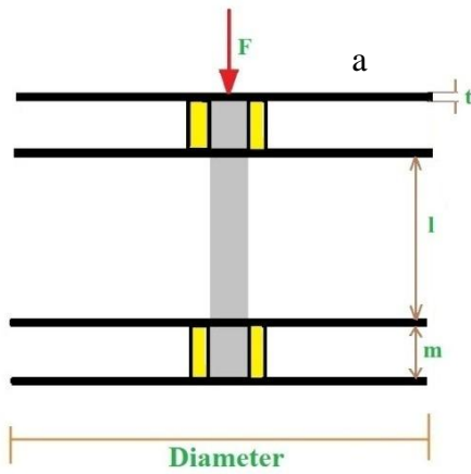
Figure 2: (a) Assembly of 3 arm flexural disc for z-stage; (b) FE Analysis of flexural z-stage.
