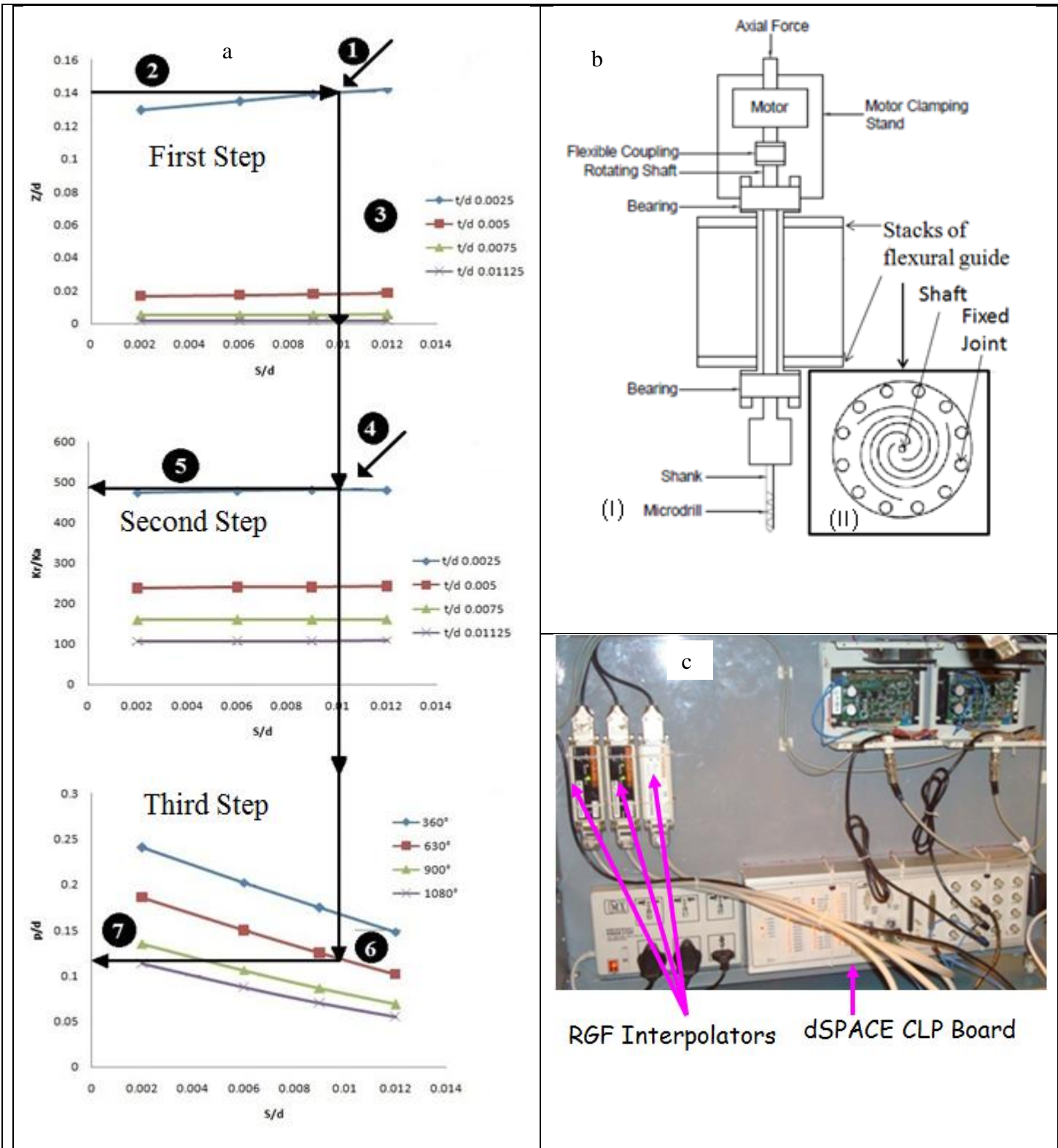
Figure 4. (a) Design method example for two layer three arm flexure system with Z/d=0.14 (b) Schematic of flexural z-stage of micro-milling (c) RGF interpolators of encoders and dSPACE 1104 DAQ platform.
