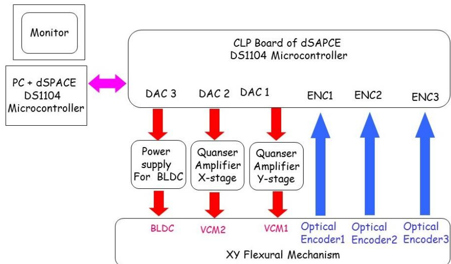
Figure 3: System integration for micro-milling workstation.
