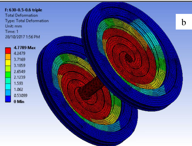
Figure 2: (a) Assembly of 3 arm flexural disc for z-stage; (b) FE Analysis of flexural z-stage.
